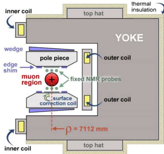
Fig. 3. Cross section of an E989 magnet.
