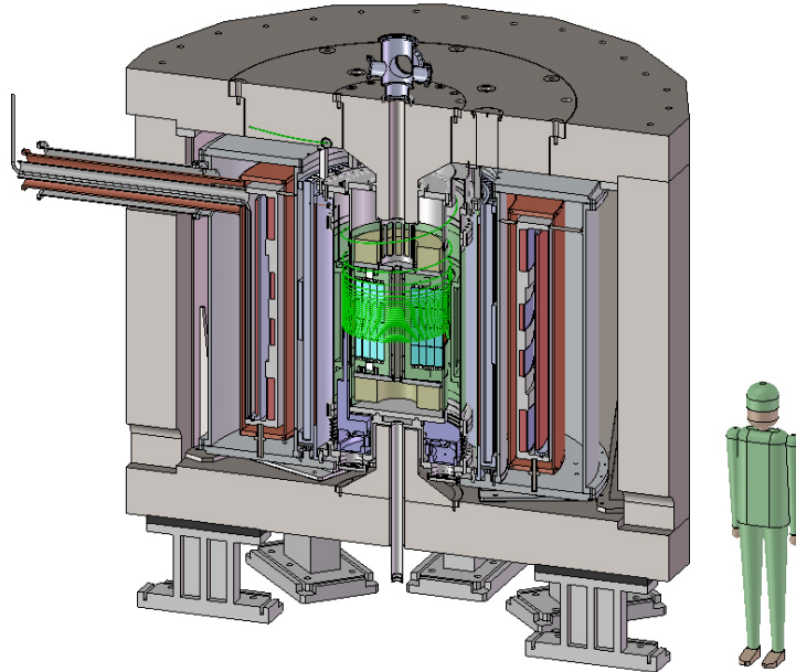
Fig. 4. The proposed setup for the J-PARC g - 2 Experiment. Muons enter at the top left (green trajectory) and spiral into the highly uniform magnetic field region. Their decay positrons curl inward to an array of silicon tracking detectors. Courtesy of T. Mibe.
