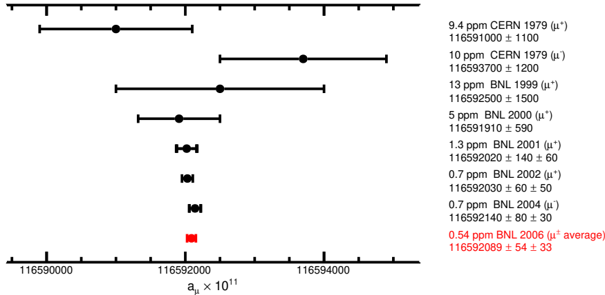
Fig. 1. Experimental measurements of a_\mu since 1979.
